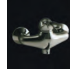
Art. 548/E MISCELATORE MONOCOMANDO DOCCIA ESTERNO Duplex con flessibile mm. 1500, eccentrici da 1/2 " regolabili per interasse da mm. 150 ± 15 EXTERNAL SINGLE LEVER SHOWER MIXER Duplex with shower hose mm. 1500, s-tailpieces with 1/2" connections, centre distance mm 150 ± 15
